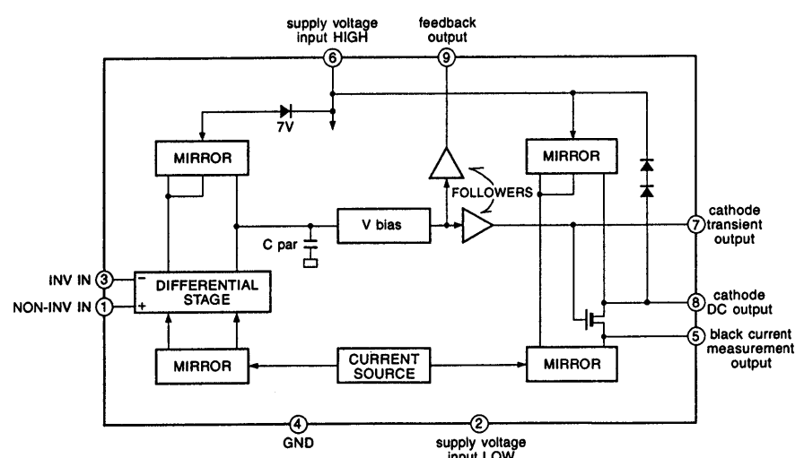
C BOARD IC701, 702, 703 TDA6101Q/N3
